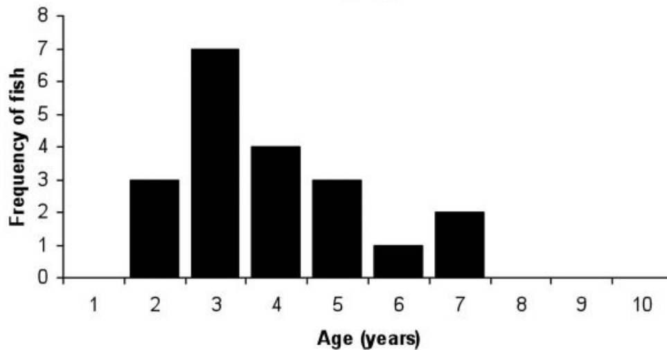
Australian herring age structure
